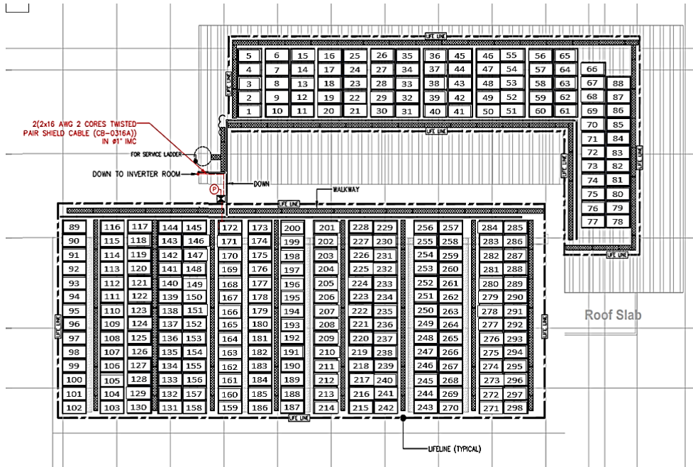
Layout T0007
