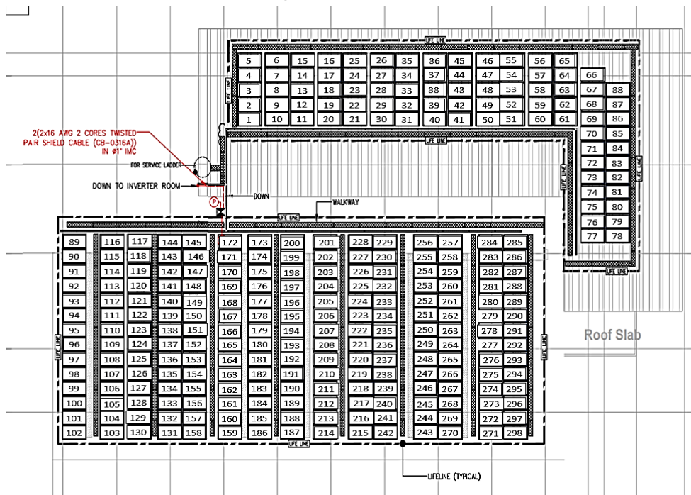
Layout T0007
