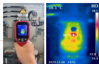
breaker inverter No.2 38.5 °C
