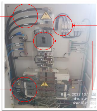
PV AC DB No.1 07NPB-WAC01
