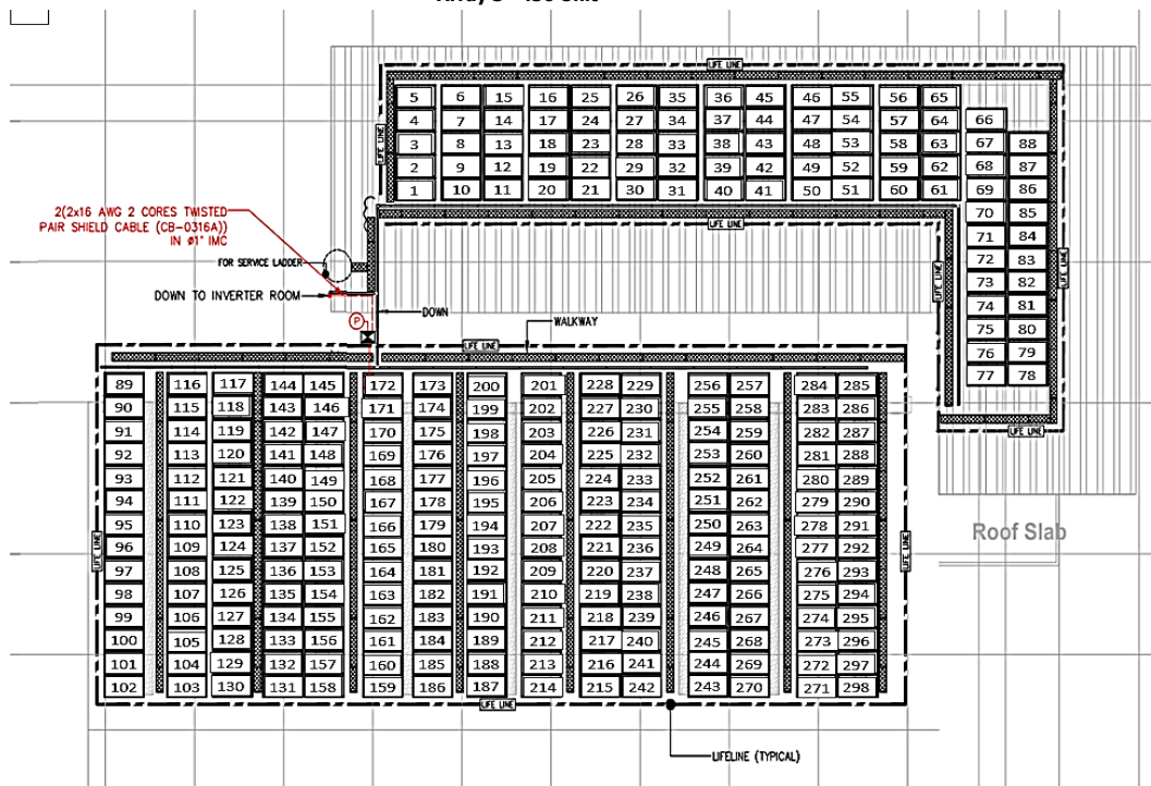
Layout T0007
