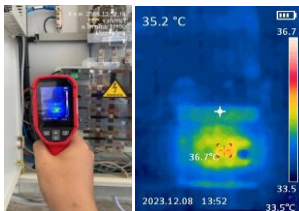
breaker inverter No.1 36.7 °C
